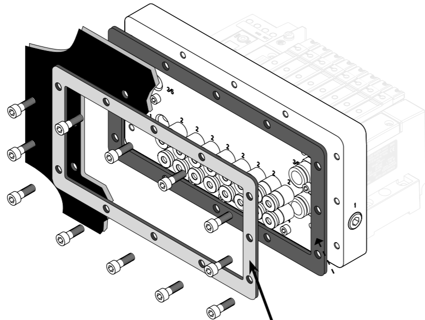
External Mounting Flange (AISI 316L)
