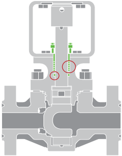
STEM SEALING
