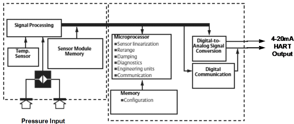
Figure 1 3051, Parts included in the FMEDA
