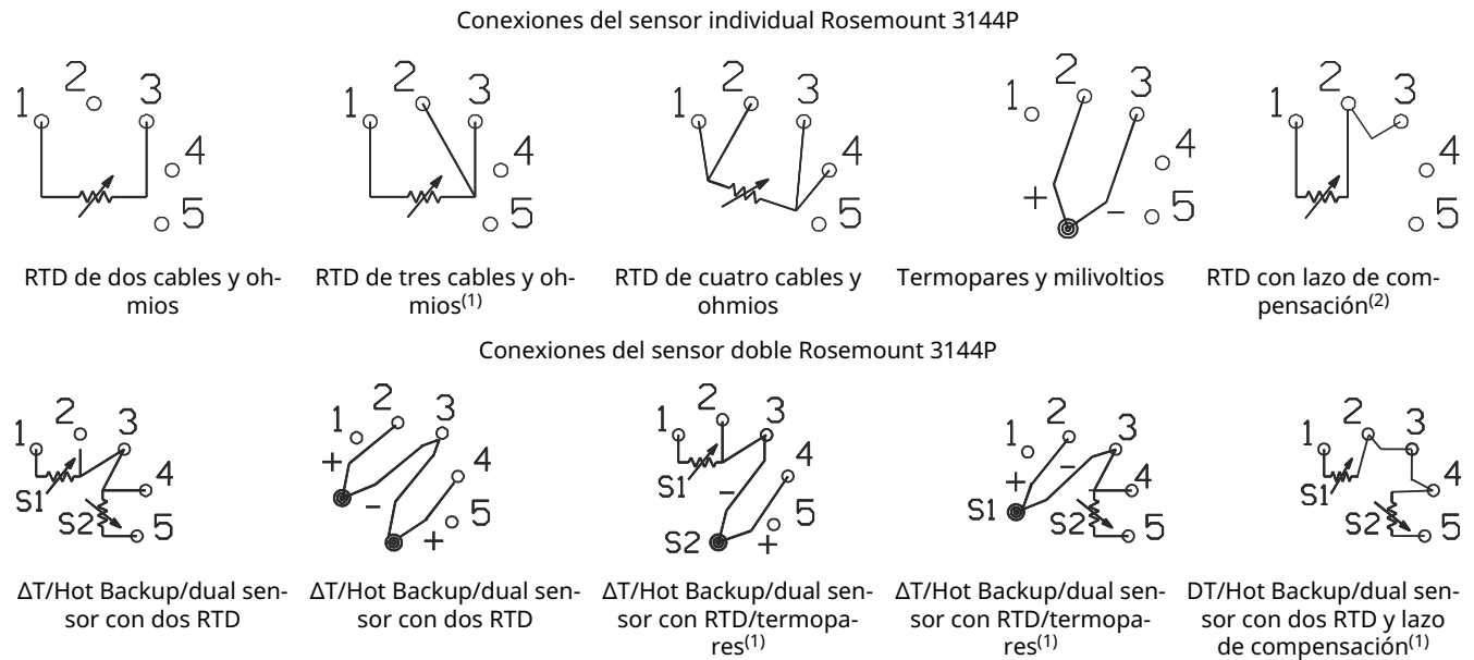
Figura 8: HART®/4–20 mA
