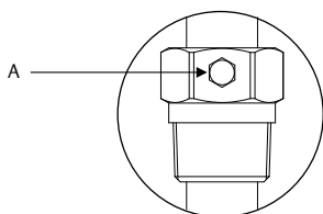
Figur 2-2: Glidemuffe, M8-skruer
