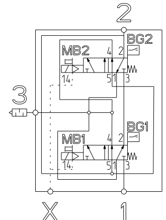
4 Schaltbild Varianten R422003730, -982, interne Vorsteuerung (links) und R422003729, -980, externe (rechts) Vorsteuerung | Schéma pneumatique variantes R422003730, -982, pilotage interne (gauche) et R422003729, -980, pilotage externe (droite) | Wiring diagram for variants R422003730, -982, internal pilot (left) and R422003729, -980, external pilot (right) | Varianti schema di collegamento R422003730, -982, pilotaggio interno (a sinistra) ed R422003729, -980 pilotaggio esterno (a destra) | Diagrama de conexiones variantes R422003730, -982, pilotaje previo interno (izquierda) y R422003729, -980 pilotaje previo externo (derecha) | Kopplingsschema varianter R422003730, -982, intern pilotmatning (vänster) och R422003729, -980, extern pilotmatning (höger)
