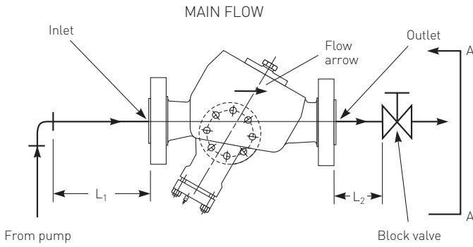
INSTALLATION DIAGRAM
