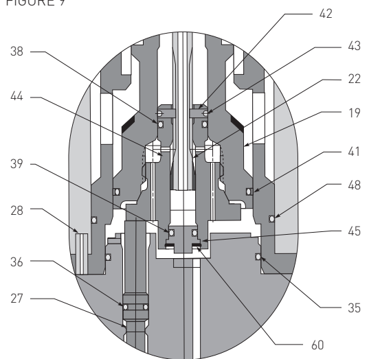
DETAIL C
