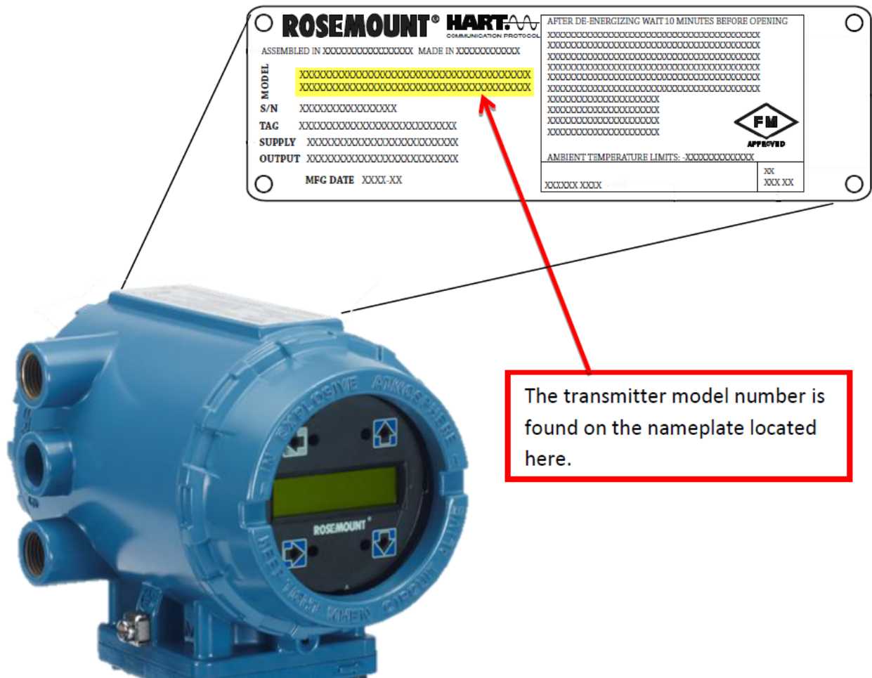
Figure 1. Transmitter Nameplate Location
