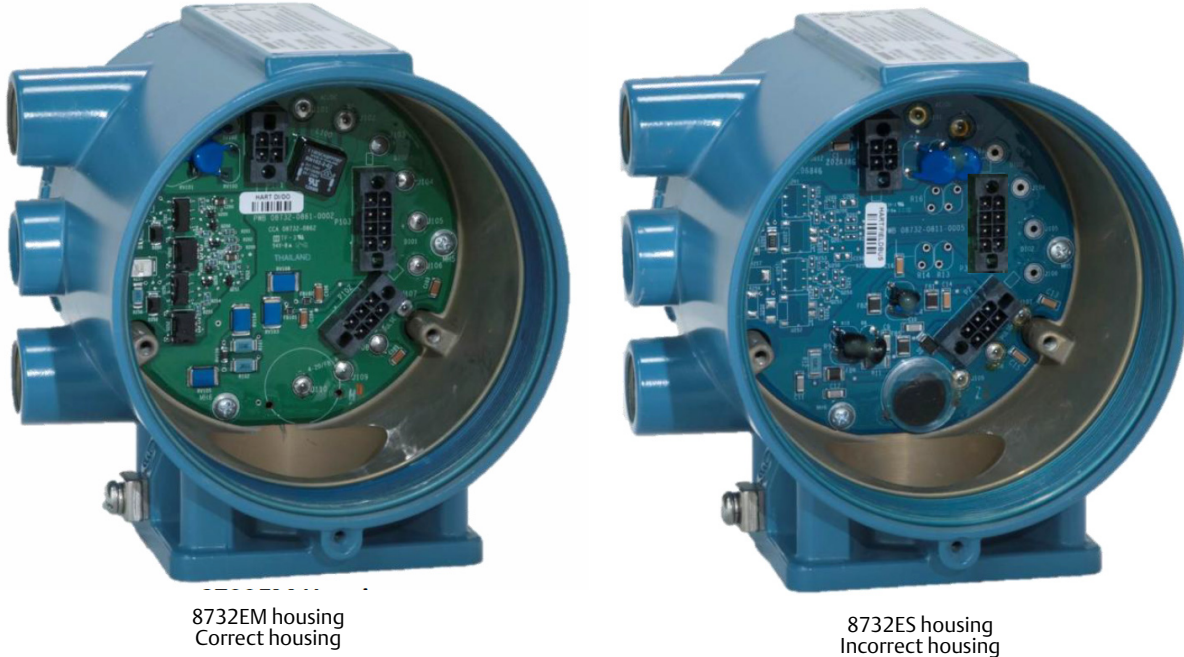
Figure 2. Transmitter Housing Electronics Board Identification
