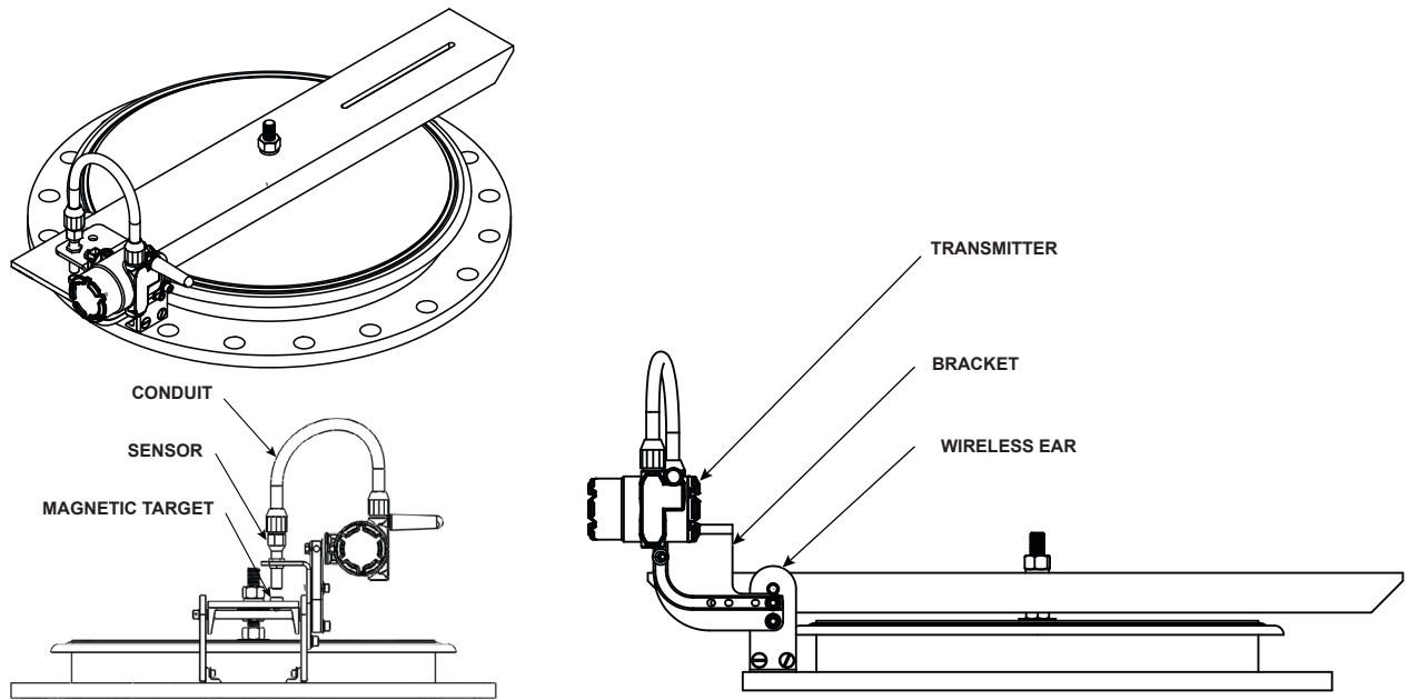
Figure 8. Enardo 2000 Smart Wireless Monitoring Option
