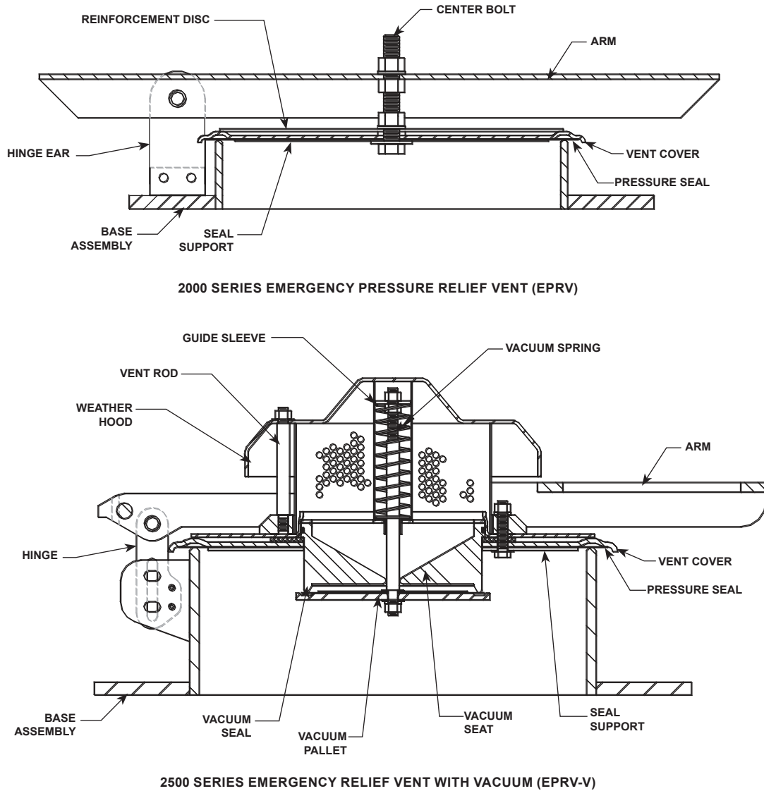
2000 SERIES EMERGENCY PRESSURE RELIEF VENT (EPRV) 2500 SERIES EMERGENCY RELIEF VENT WITH VACUUM (EPRV-V)
