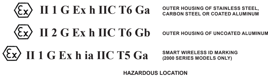
Figure 4. Product Identification and Marking
