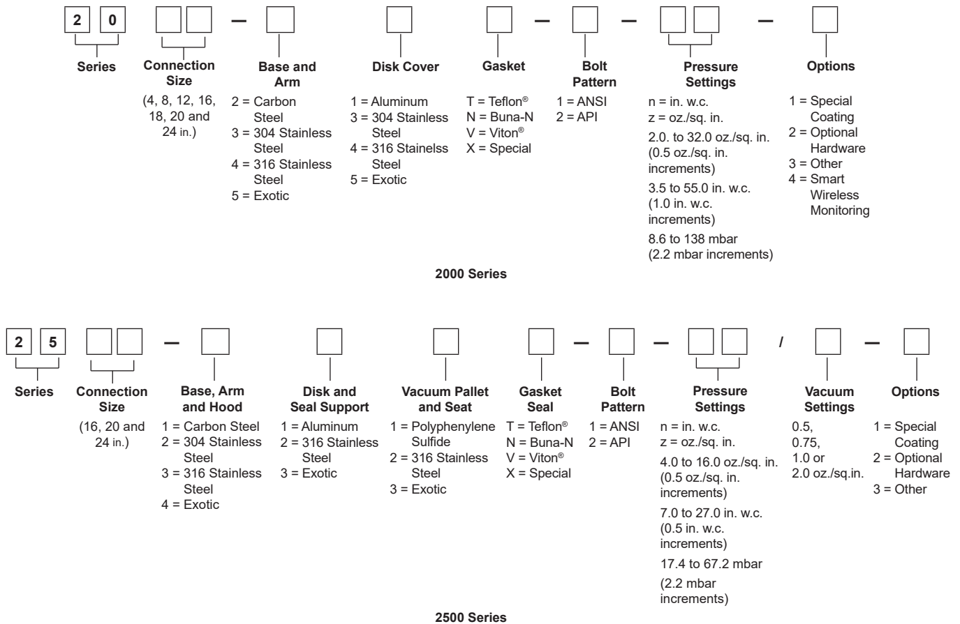
Figure 5. Emergency Pressure Relief Vent Model Number
