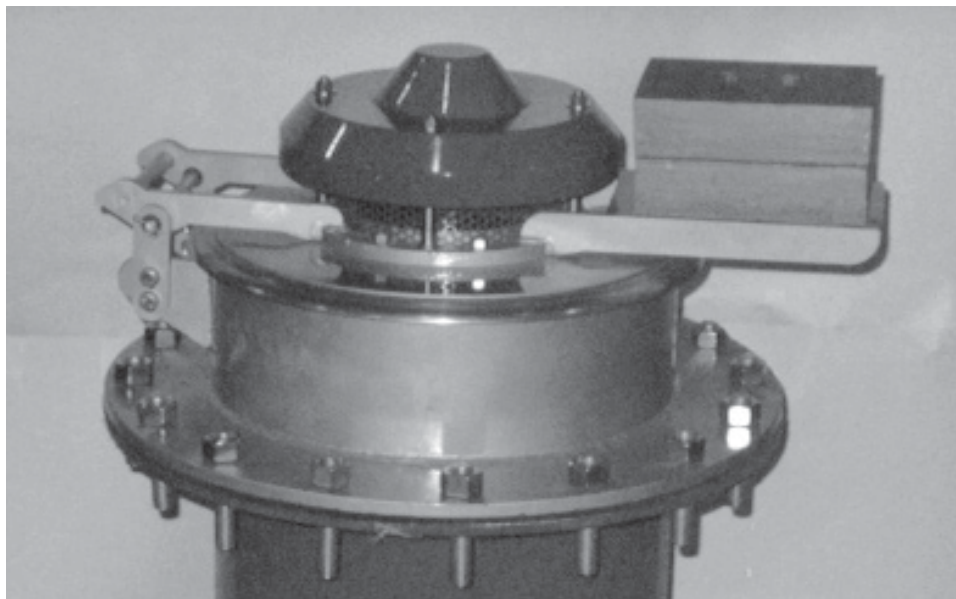
Figure 9. 2500 Series with an Elevated Pressure Setting
