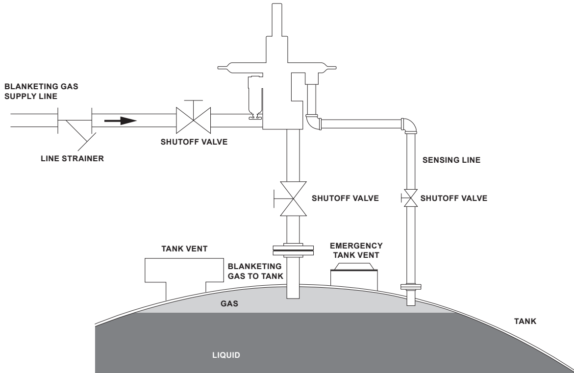
Figure 4. ACE95 Series Tank Blanketing Valve Installation
