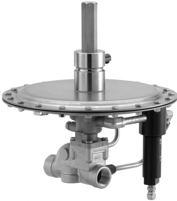
Figure 1. Type ACE95 Tank Blanketing Valve
