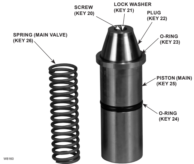
Figure 7. Typical Main Valve and Spring (Type ACE95Sr shown)
