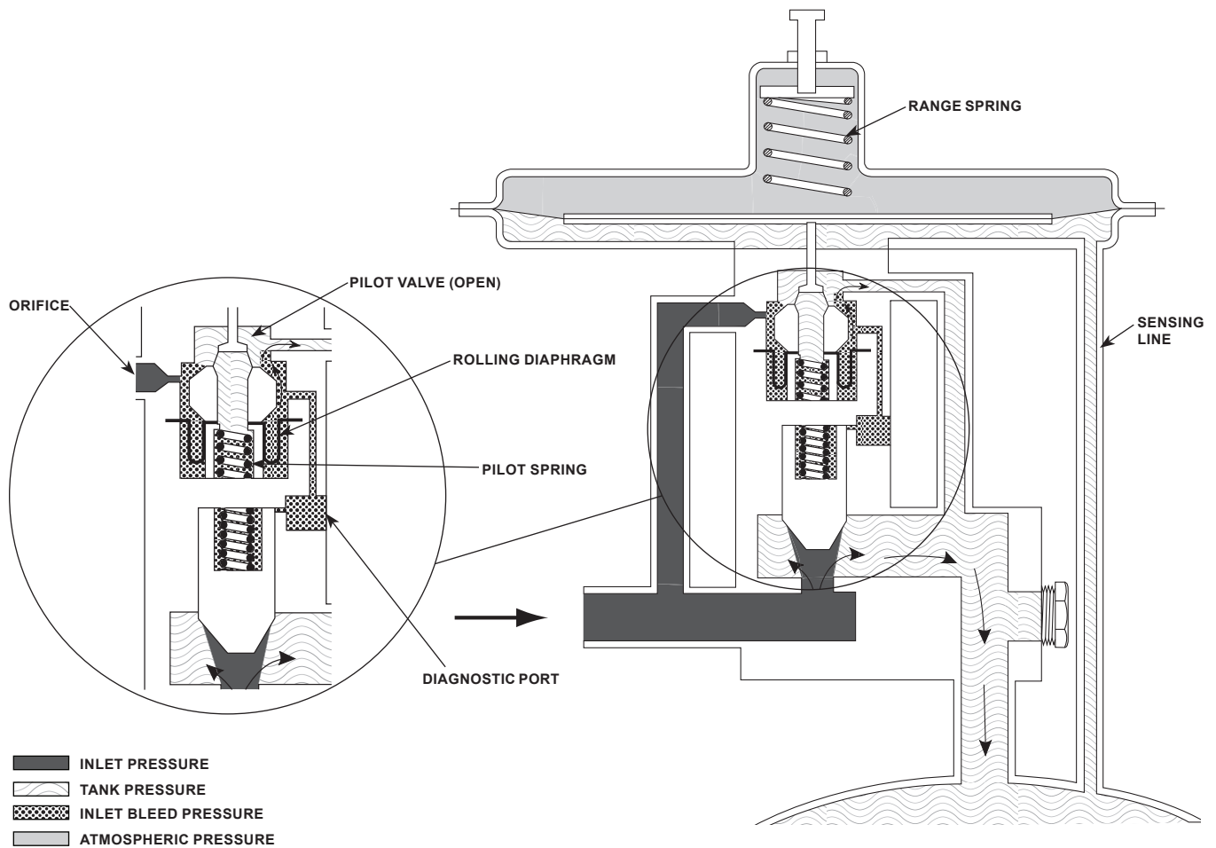
Figure 3. ACE95 Series Operational Schematic (Valve Open)
