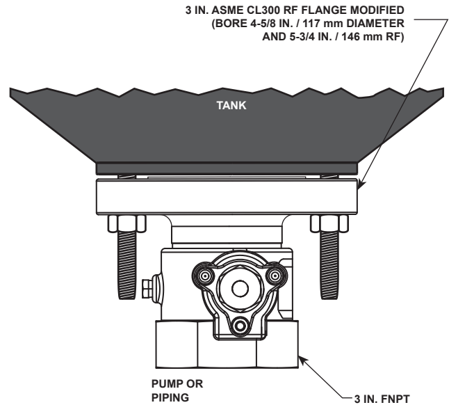
Figure 4. Valve Installation Schematic
