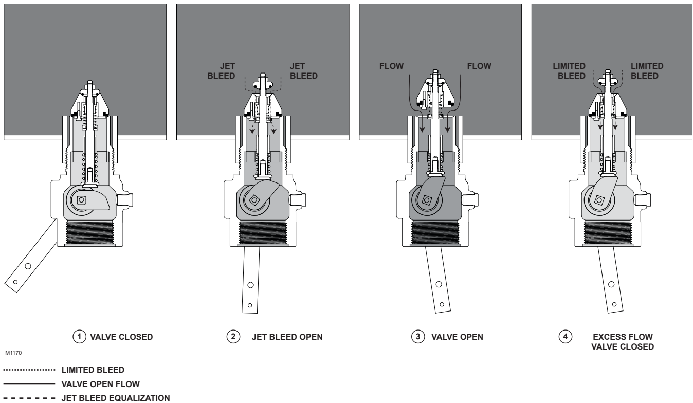
Figure 2. Operational Schematic
