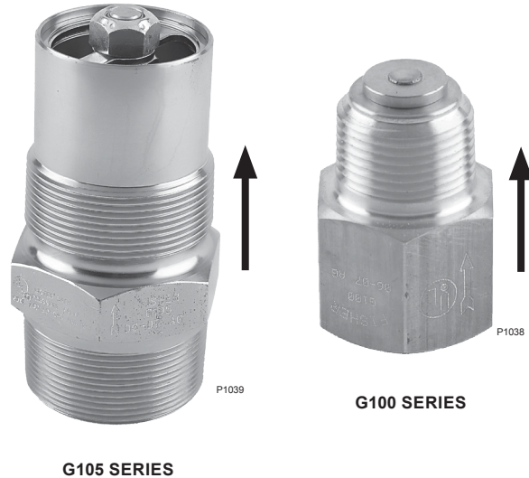
Figure 1. G100 Series Back Check Valves (Arrow indicates direction of flow)
