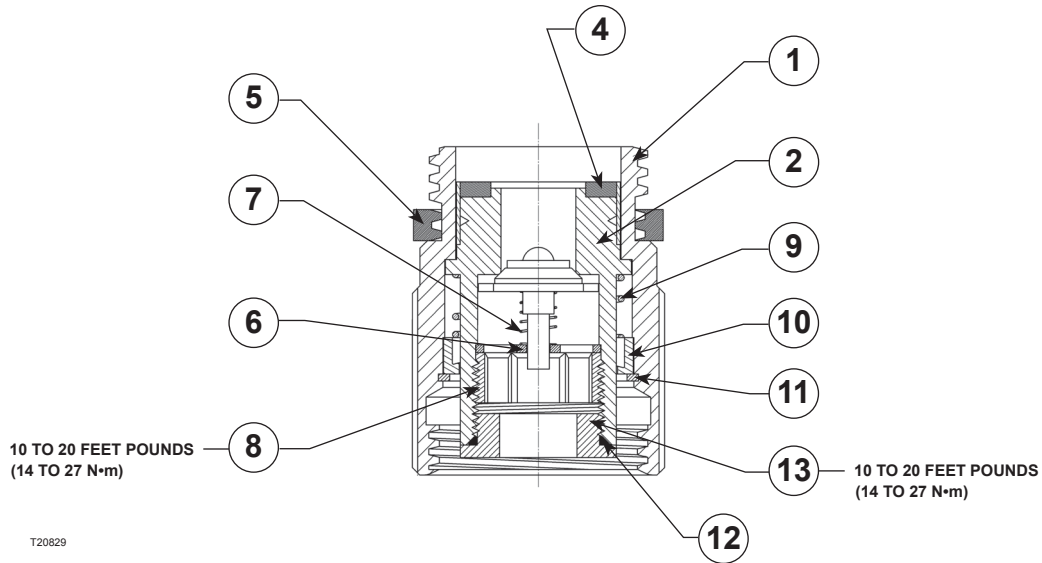
Figure 2. Type M570 Hose Adaptor Assembly
