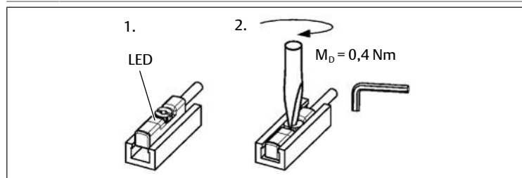
Fig. 2: Installing sensors
