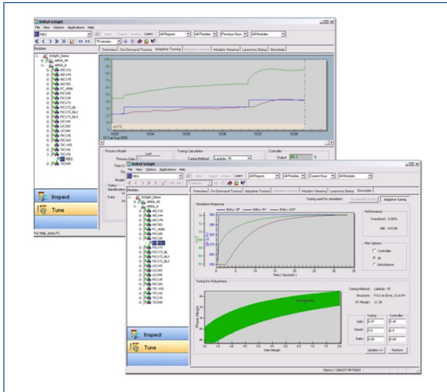
InSight Adaptive Tuning and Simulation.
