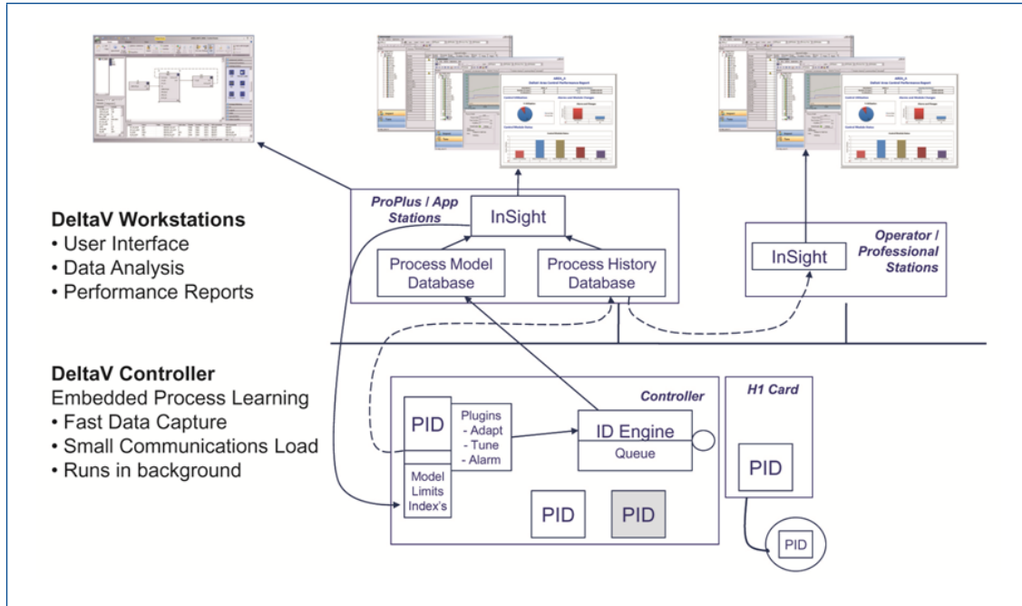
DeltaV InSight Architecture.
