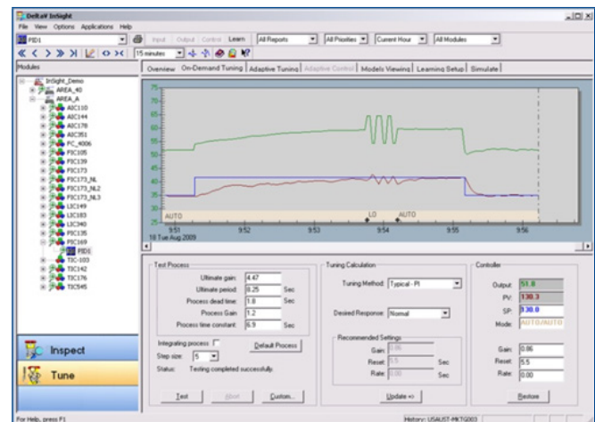
InSight On-demand Tuning.
