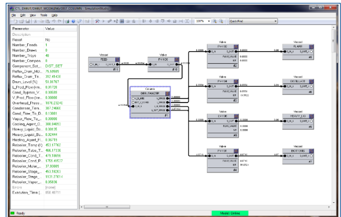
High Fidelity distillation column simulation in the Mimic Simulation Studio.
