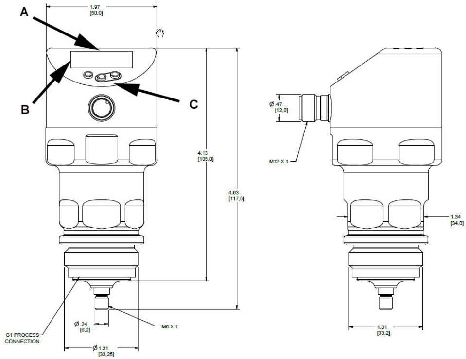
Figure 2: Rosemount 326L Level Transmitter dimensional drawing
