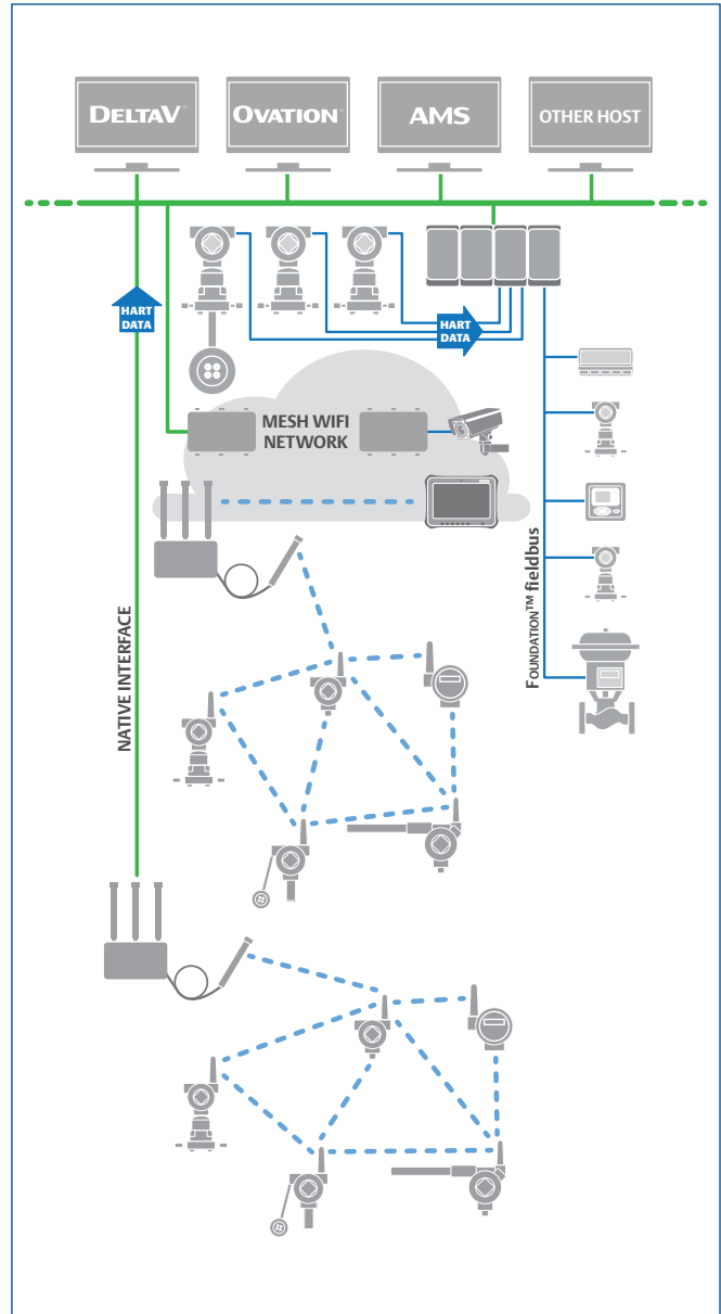
System Architecture with the 1552WU Gateway.
