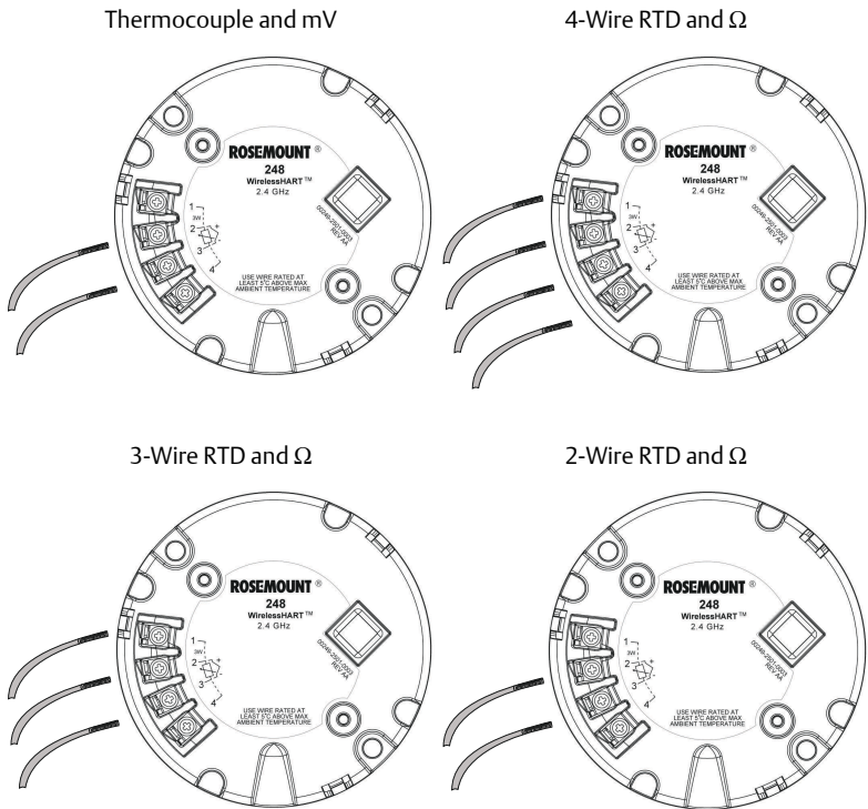
Figure 5-1: Sensor Wiring
