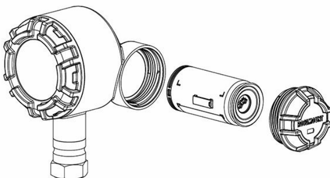
Figure 6-1: Exploded Power Module View
