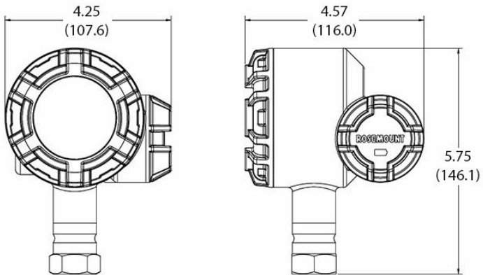
Figure 3-2: Direct Mount
