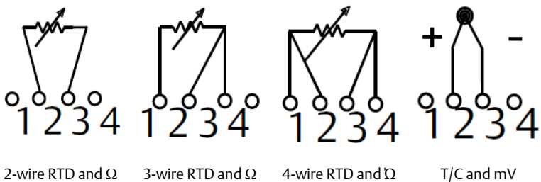
Figure 5-2: Sensor Connections
