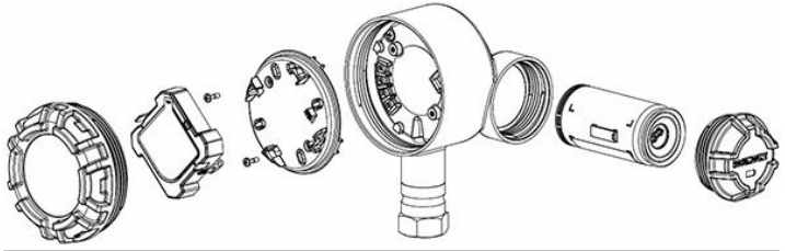
Figure 3-3: Exploded View of LCD Display Assembly
