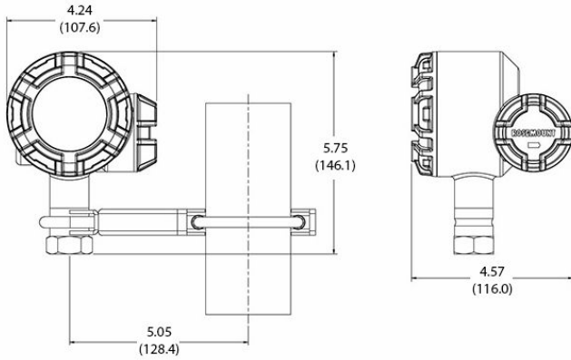
Figure 3-4: Remote Mount
