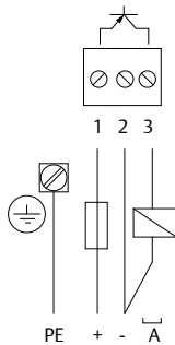
Figure 3-4: Power Supply and Signal Output (Three-wire PNP)
