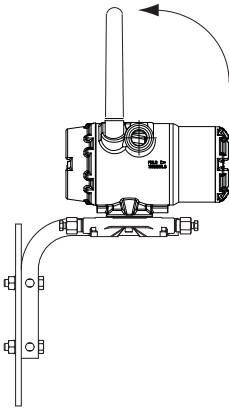
Figure 1. Antenna Position
