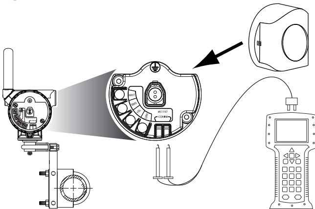
Figure 3. Connection
